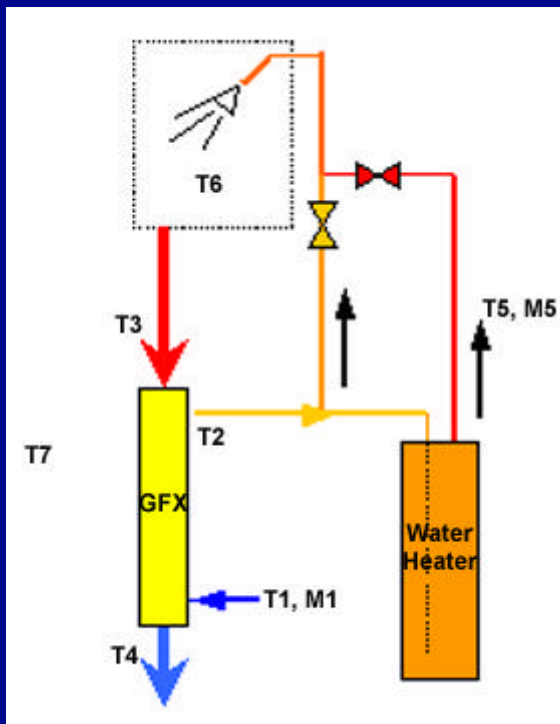
Figure 1. Layout of GFX system in residential application.
