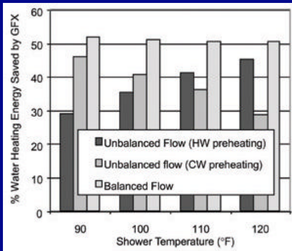
Figure 3. Energy saved using GFX according to flow.
